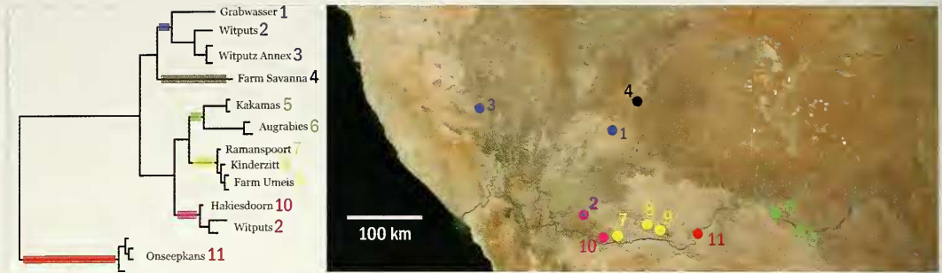
FIGURE 124. Detail of Bayesian gene tree of Pachyactylus montanus based on sequence data from a portion of the cytochrome b gene. Subclades are color-coded and localities are numbered to correspond to points plotted on the satellite image of the Orange River and adjacent areas of South Africa and Namibia. There is generally good fit between apparent relationships and geographic patterns, but specimens from Onseepkans are highly divergent from their nearest neighbors, despite exhibiting no obvious morphological differences. See text for further discussion. MODIS imagery from the Global Land Cover Facility ( http://www.landcover.org ).
